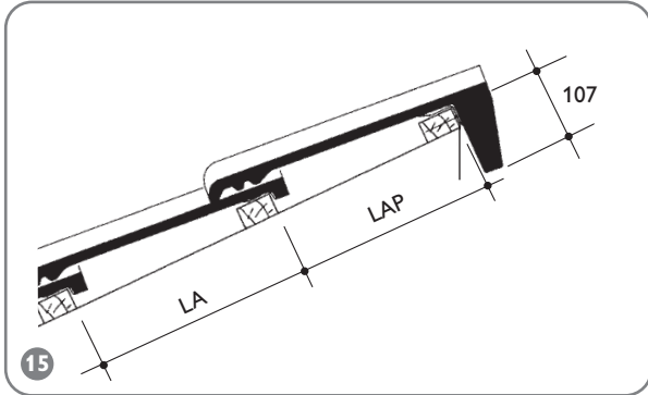
Lattenabstand-Pult (LAP) in mm Tabelle 20
